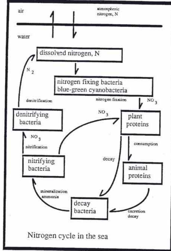
Figure 8. The nitrogen cycle in seawater.
