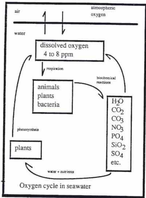
Figure 7. The oxygen cycle in the sea and in marine aquariums.
