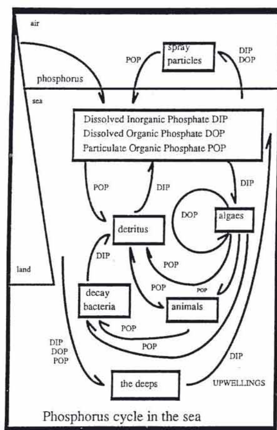
Figure 10. Phosphorus cycle in seawater.
